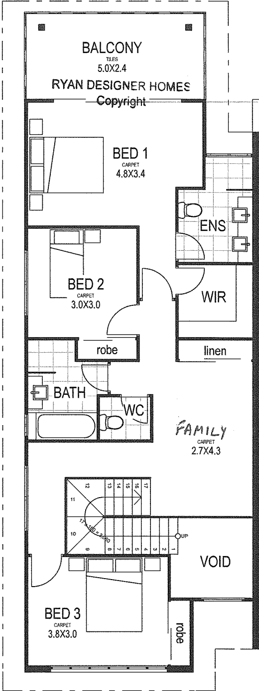
Upper Level Floor Plan
