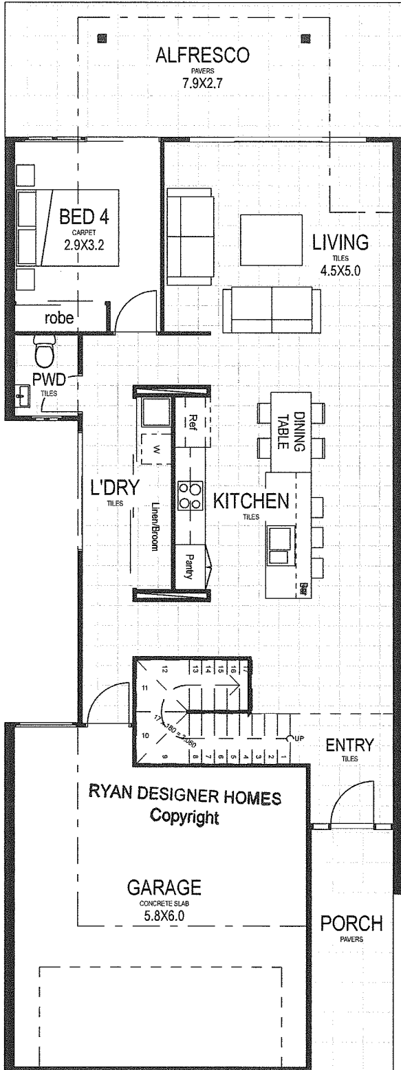
Ground Level Floor Plan
